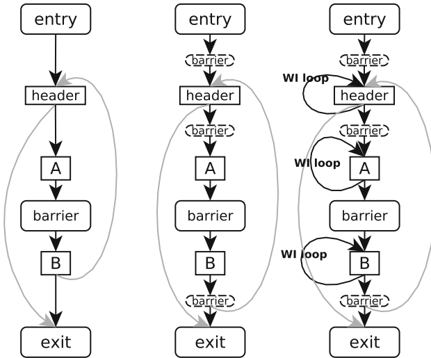
Fig. 8 Adding implicit barriers to kernels with b-loops to produce unambiguous parallel regions; a the original single work-item kernel CFG with the b-loop, b the kernel CFG with implicit barriers added to make parallel region formation unambiguous, and c the work-group function CFG with the work-item loops added to iterate the parallel regions. The original kernel loop edges are colored grey
