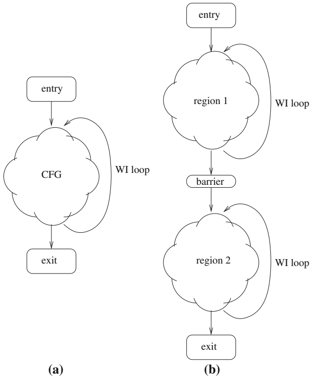
Fig. 4 Two basic cases of static work-group function generation: A kernel a without work-group barriers and b with an unconditional barrier in the middle
