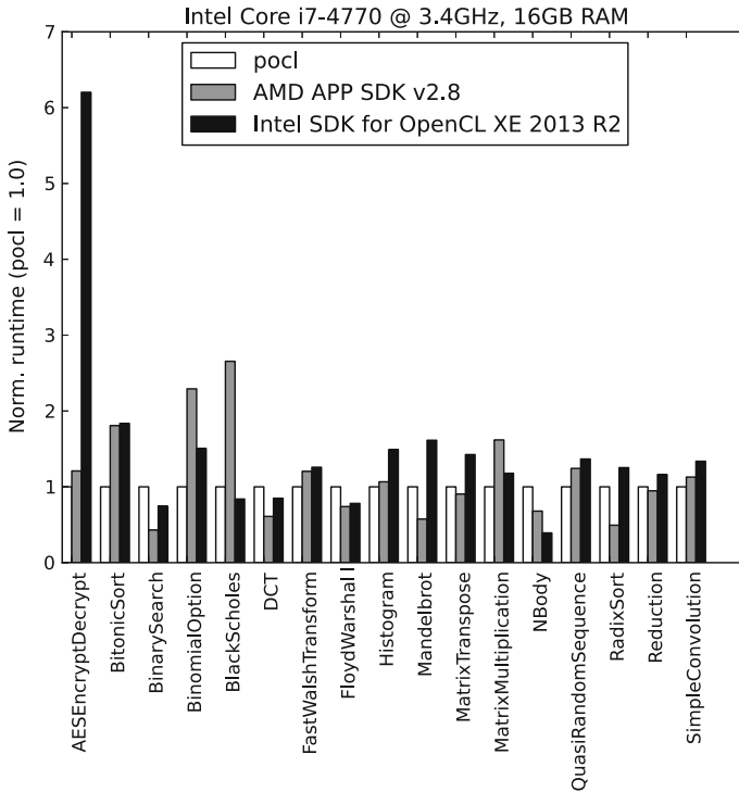
Fig. 12 Benchmark execution times (smaller is better) with Intel Core i7, in a Linux environment. The benchmark runtime achieved with pocl is compared to the two available proprietary implementations for the platform
