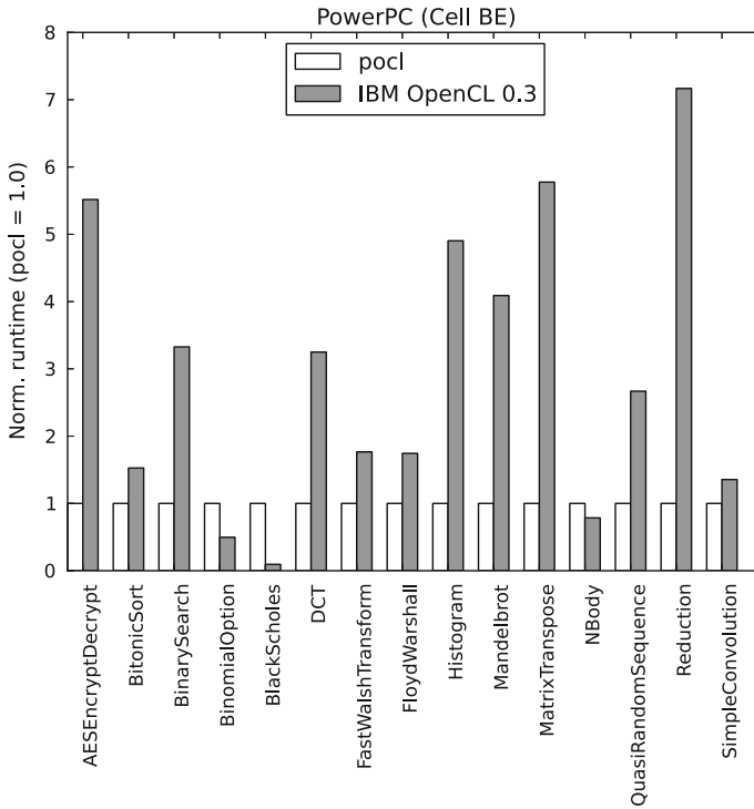
Fig. 14 Benchmark execution times ( smaller is better ) with STI CellBE @ 3.2GHz, 256MB RAM running Debian sid. Both OpenCL implementations utilize the PowerPC processor only
