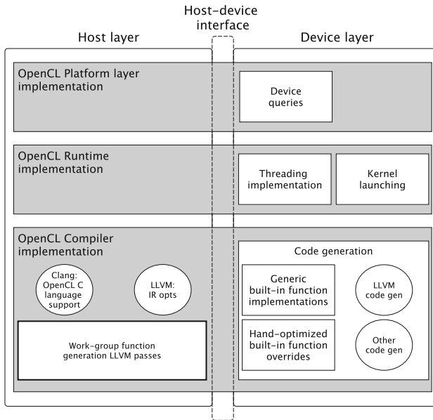
Fig. 2 The subcomponents in the OpenCL implementation. The host layer includes parts that are executed in the OpenCL host. The device layer is used as a hardware abstraction layer to encapsulate the device-specific parts
