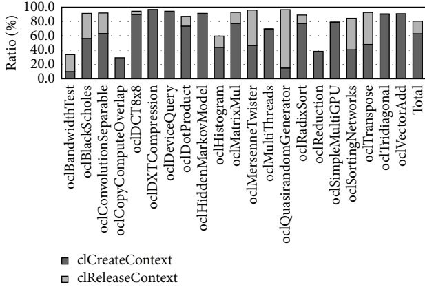
FIGURE 6: Execution time distribution of cICreateContext and cIReleaseContext .
